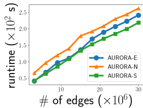
Fig. 11: running time vs. the number of edges on Pokec dataset
