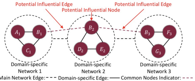
Fig. 1: Example of potential influential edges and node in Network of Networks model.
