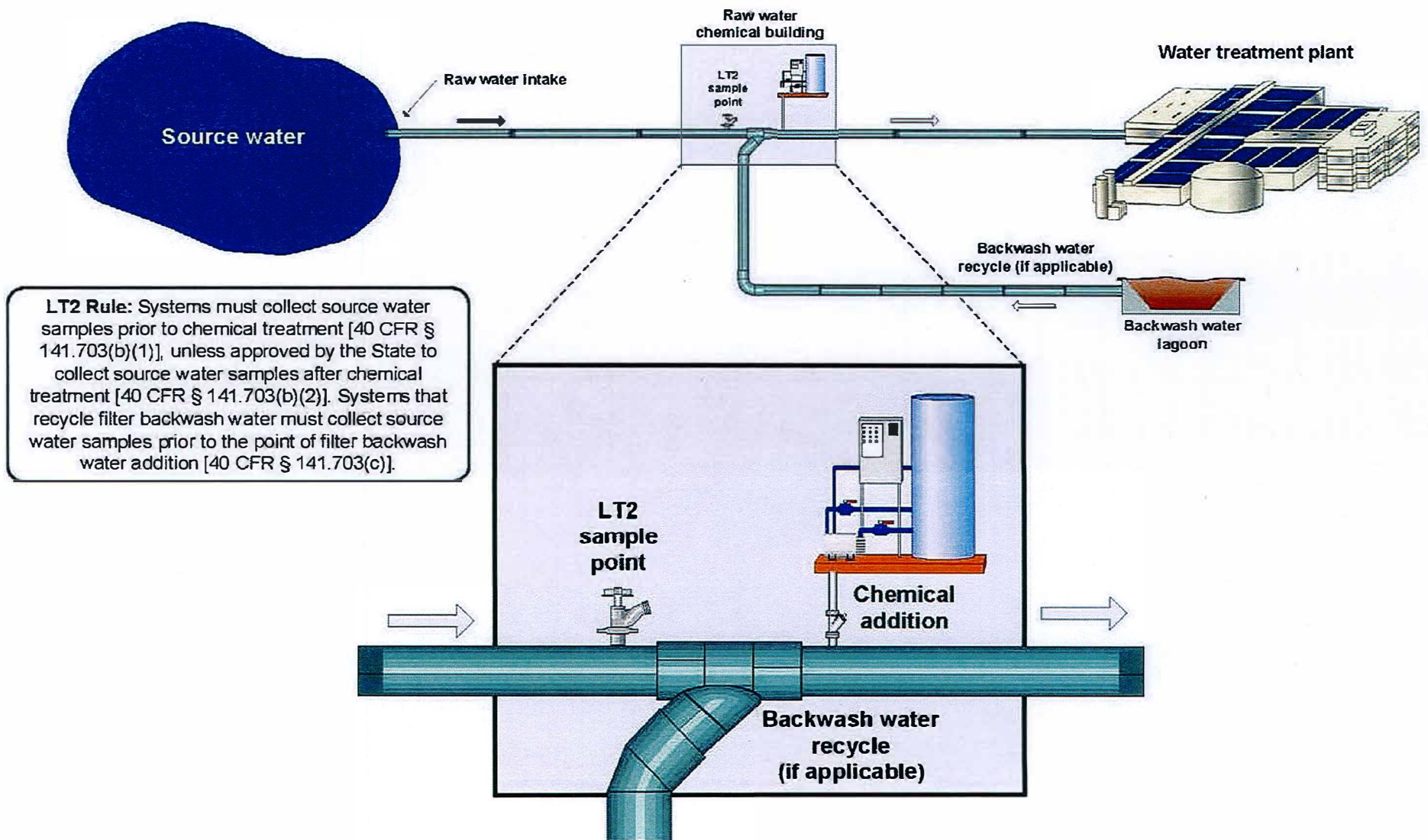
Figure 1. Sample Tap before Chemical Treatment and Backwash Water Recycle (if applicable)
