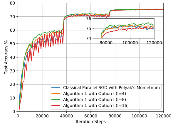
(b) Test accuracy v.s. iteration steps.
