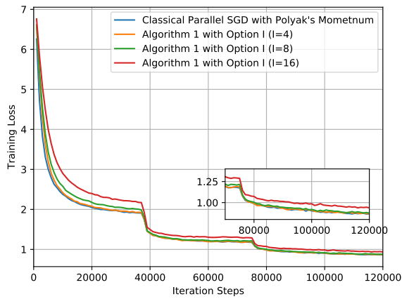
(a) Training loss v.s. iteration steps.
