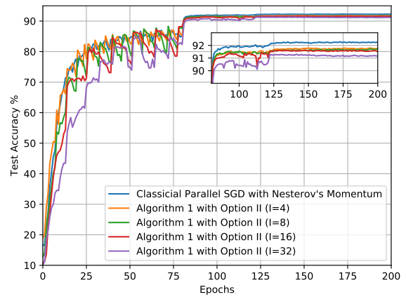
(b) Test accuracy v.s. epochs.
