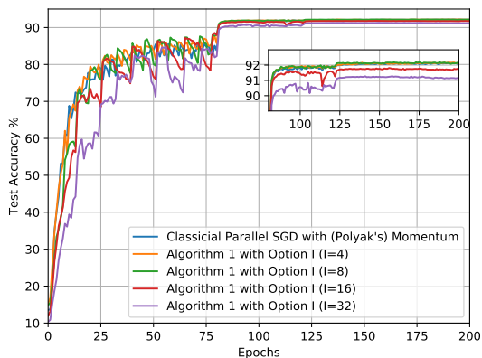
(b) Test accuracy v.s. epochs.
