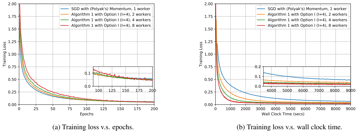
Figure 4: Algorithm 1 with constant learning rates: linear speedup verification with ResNet56 over CIFAR10.
