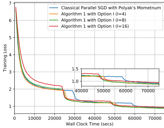
(a) Training loss v.s. wall clock time.
