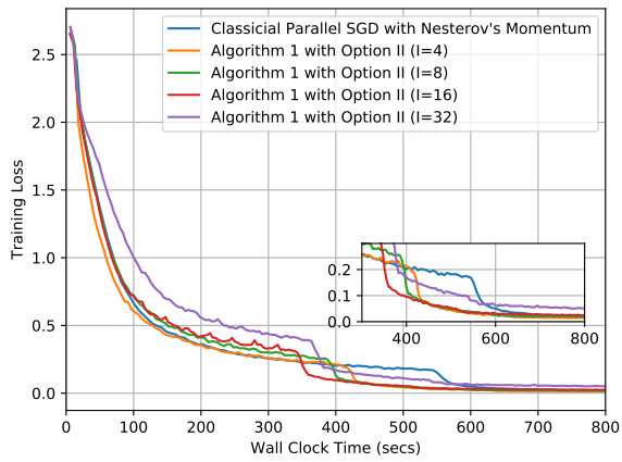
(a) Training loss v.s. wall clock time.
