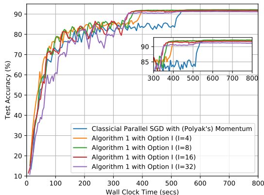
(b) Test accuracy v.s. wall clock time.
