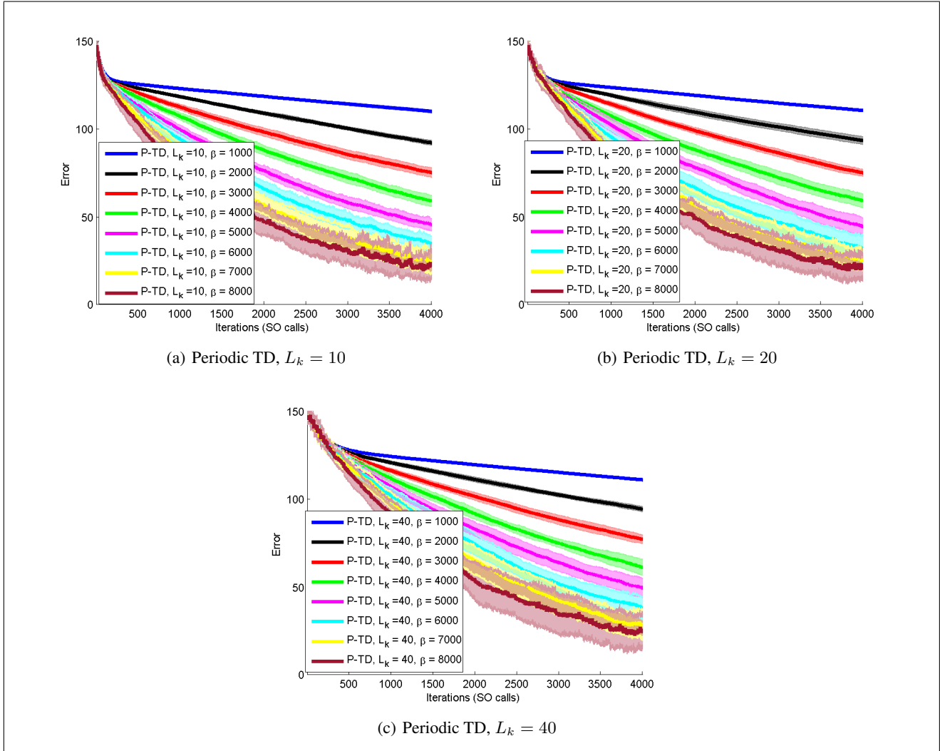
Figure 6: Error evolution of P-TD with different step-sizes, \beta_t = \beta / (10000 + t) , \beta = 1000, 2000, \dots, 8000 . Each subplot uses different L_k : (a) L_k = 10 ; (b) L_k = 20 ; (c) L_k = 40 . The shaded areas depict empirical variances obtained with several realizations.
