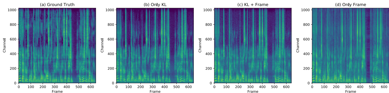
Figure 4. Spectrogram visualization of ClariNet samples with different loss configurations.
