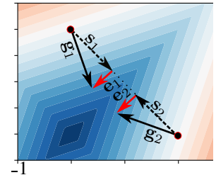
Figure 1: The gradients \mathbf{g} (in solid black), signed gradient direction \mathbf{s} = \text{sign}(\mathbf{g}) (in dashed black), and the error \mathbf{e} (in red) are plotted for \epsilon = 0.5 . SIGNSGD moves only along \mathbf{s} = \pm(1, -1) while the error \mathbf{e} is ignored.
