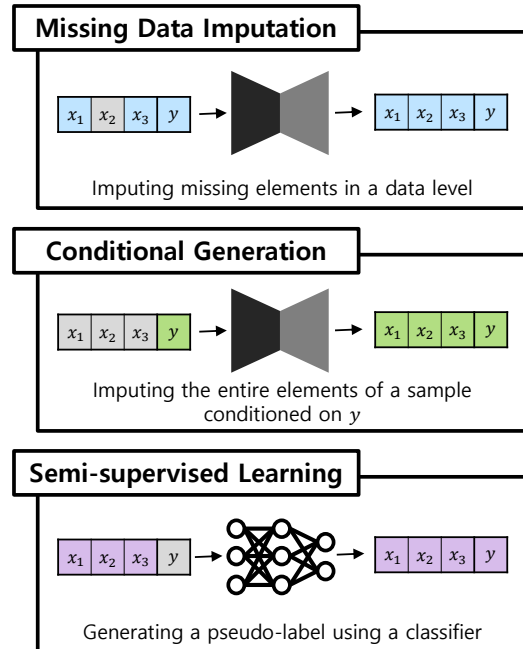
Figure 1. Tasks for the three main problems in real world classification. We define missing data imputation as a task that fills in missing data elements. Conditional generation can be defined as a task that imputes the entire elements in an instance conditioned on a certain class. Semi-supervised learning can be defined as a task that imputes missing labels.
