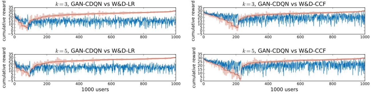
Figure 4. Cumulative rewards among 1,000 users under the recommendation policies based on different user models. The experiments are repeated for 50 times and the standard deviation is plotted as the shaded area.
