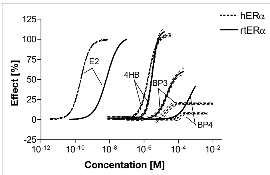
Fig. 1. Estrogenic activity of UV filters in the human hERα and rainbow trout rtERα recombinant yeast assay. E2, Estradiol; 4HB, 4-hydroxy benzophenone; BP3, benzophenone-3; BP4, benzophenone-4. [24]
