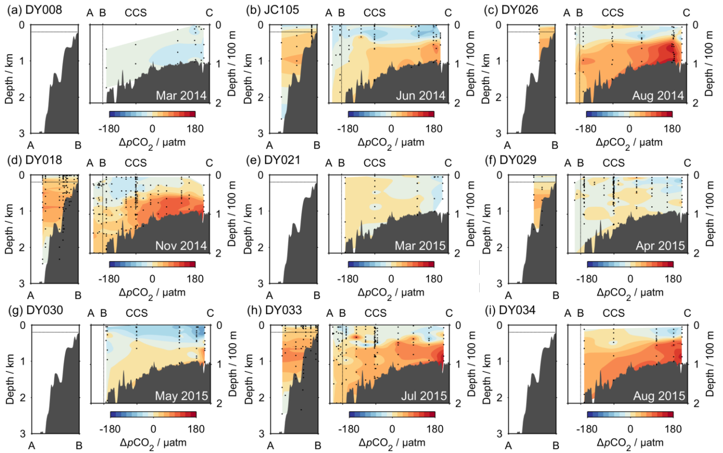
Figure S7. Transects of \Delta p\text{CO}_2 , calculated from C_T and A_T measurements, across the Celtic Sea for each SSB cruise. The layout is as described for Fig. 7.
