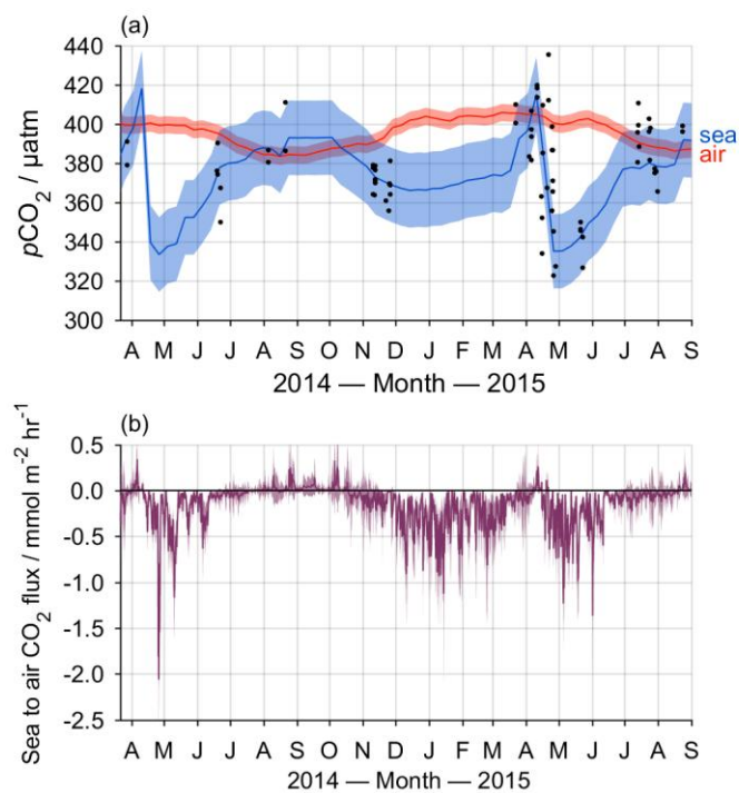
Figure 2. Time-series of air-sea \text{CO}_2 disequilibrium and flux at CCS. (a) Atmospheric (red) and sea surface (blue) p\text{CO}_2 at CCS. The black points show the actual measurements of surface p\text{CO}_2^{\text{sw}} , while the blue line shows our algorithm-predicted interpolation of these data (Table 2) that was used to calculate \Delta p\text{CO}_2 and then the air-sea \text{CO}_2 flux. (b) The sea to air \text{CO}_2 flux. The shaded areas show the 95% confidence intervals.
