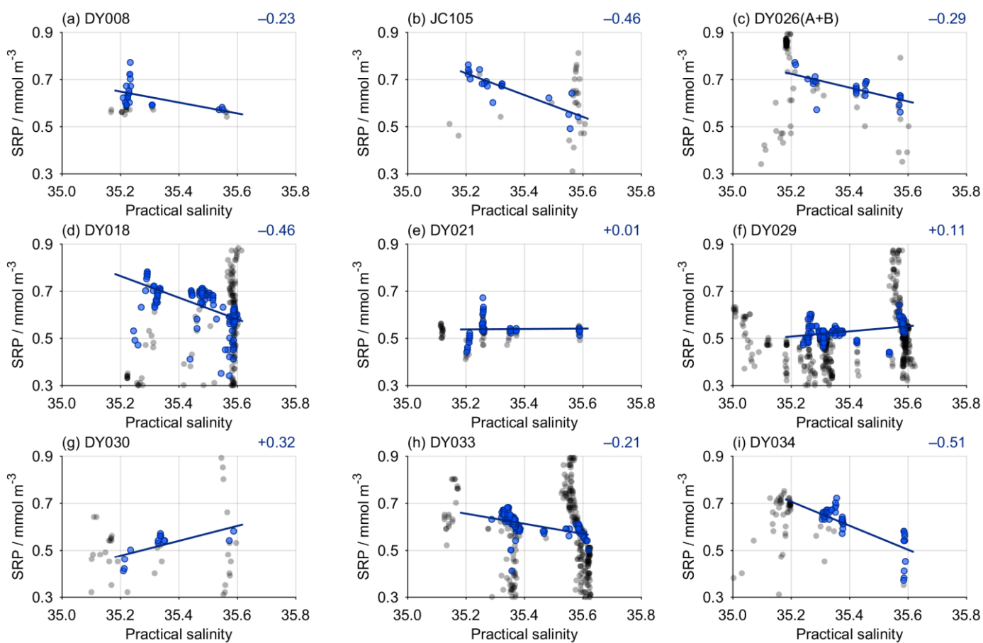
Figure S14. Relationship between soluble reactive phosphorus (SRP) and practical salinity for each UK-SSB cruise. The points used to generate each regression are shown in blue (Section 2.8), and the slope is indicated towards the top right of each panel (see also Fig. 7 and Table 3).
