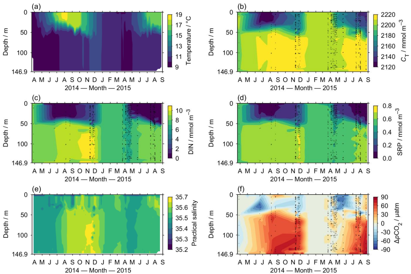
Figure 3. Hovmöller diagrams of CCS water column (a) temperature, (b) dissolved inorganic carbon, (c) dissolved inorganic nitrogen (i.e. nitrate + nitrate + ammonium), (d) soluble reactive phosphorus, (e) practical salinity, and (f) air-sea \text{CO}_2 disequilibrium. Where shown, sampling locations are indicated as black points. The cycle of winter mixing and summer stratification is clear for most variables, while S , DIN and SRP show an anomalous increase in the deep layer during late 2014, indicating an influx of open ocean waters.
