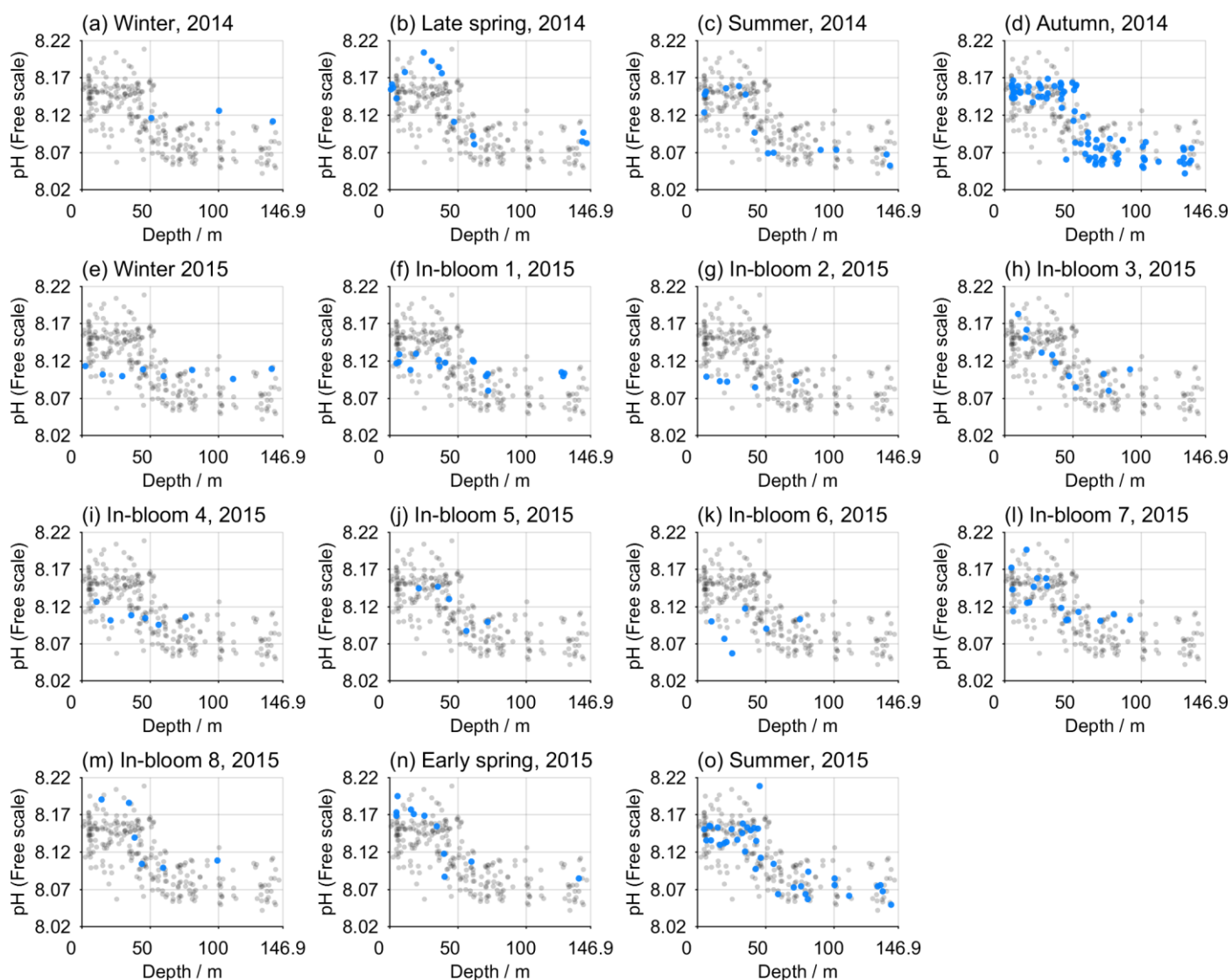
Figure S5. Seawater pH on the Free scale at each time point at CCS (Table 1), calculated from A_T and C_T measurements (van Heuven et al., 2011). The grey circles show the entire CCS dataset, while the blue circles show the data at each time point.
