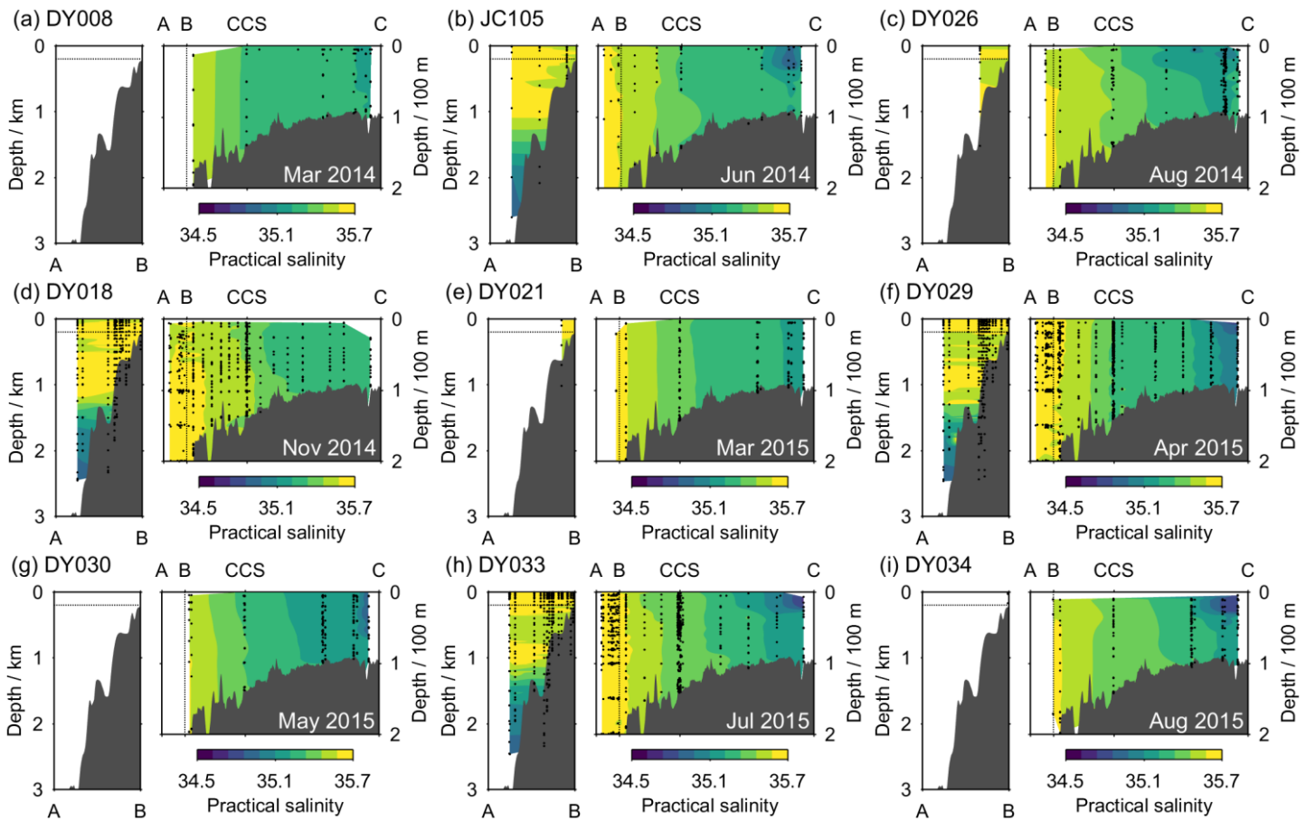
Figure S11. Transects of practical salinity across the Celtic Sea for all of the UK-SSB cruises.
