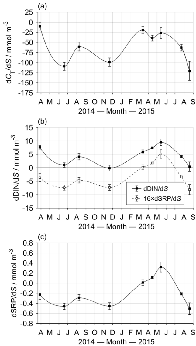
Figure 8. Time-series of regression slopes between S and (a) C_T , (b) DIN , and (c) SRP . Negative values indicate that the on-shelf deep layer is enriched in the nutrient relative to the open ocean, while positive values indicate on-shelf depletion. Error bars show the standard error in the gradient at each point (Table 3). In (b), the predicted relationship based on dSRP/dS is also shown, considered to represent the component driven by OM remineralisation. The offset between this and the solid line (mean \pm SD difference = 7.5 \pm 2.1 \text{ mmol m}^{-3} ) was likely driven by denitrification/anammox in the Celtic Sea; note that this offset value is reported per unit practical salinity (which is itself dimensionless).
