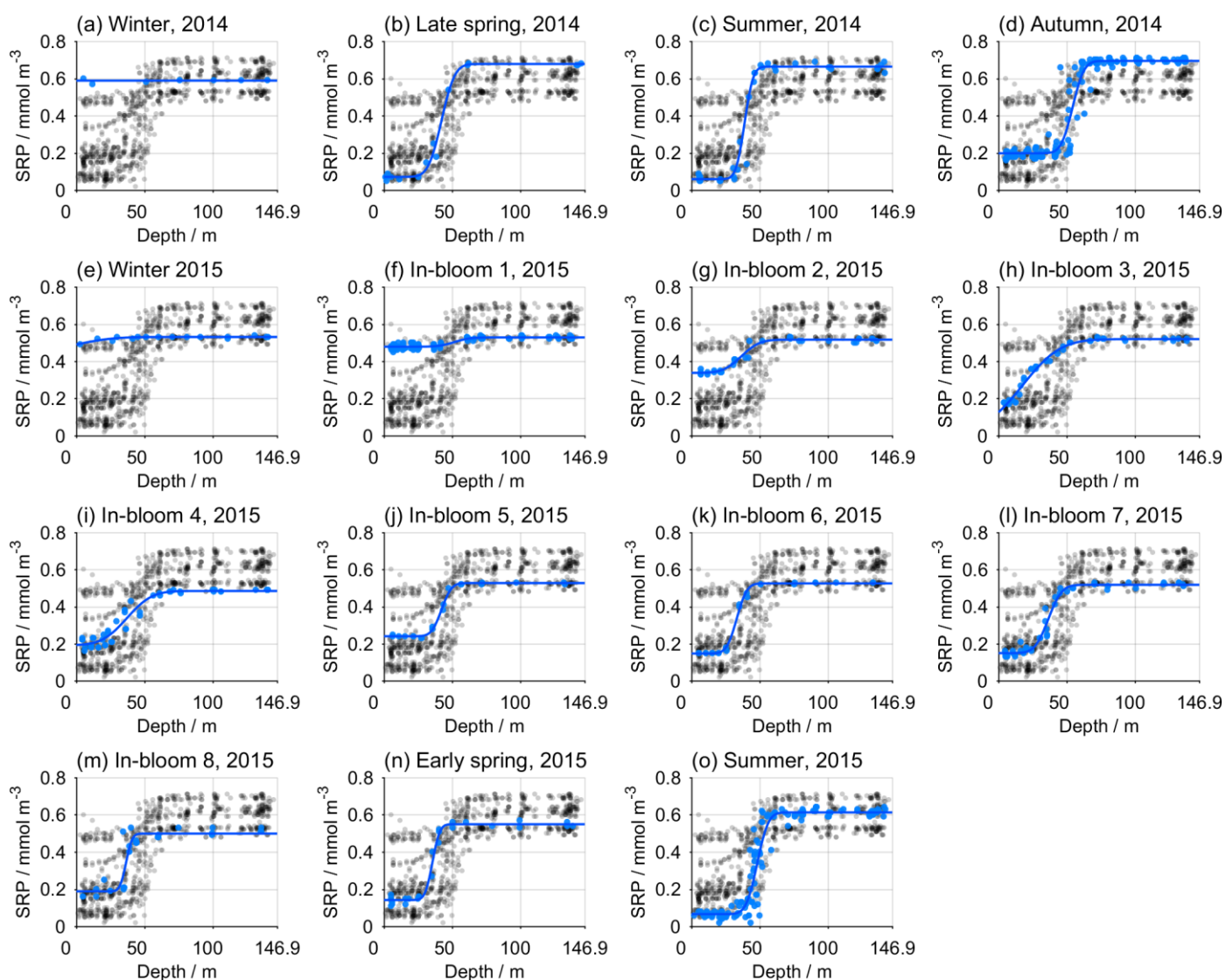
Figure S3. Soluble reactive phosphorus (SRP) profiles at each time point at CCS (Table 1).
