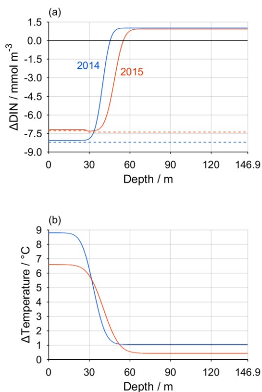
Figure 6. Winter to summer changes in (a) DIN and (b) seawater temperature for 2014 (blue) and 2015 (red). In (a), the dashed lines show the lowest possible \Delta\text{DIN} , i.e. its value if the entire winter DIN inventory had been converted into OM. All available DIN in the surface layer was converted to OM in both years. This represented a greater change in DIN in 2014 due to the higher initial DIN concentration, but the deeper nutricline in 2015 led to greater NCP overall. Remineralisation increased the deep layer DIN concentration by the same amount in both years, but this represented a smaller absolute DIN addition in 2015 owing to the deeper nutricline.
