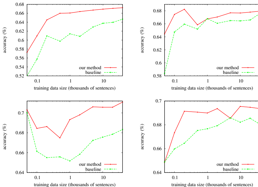
Figure 8: Learning curves. Each graph compares transferring a single tree of edges (baseline) and transferring all possible projected edges (our method). The models were trained on sentences of length up to 20 and tested on CoNLL train sentences of length up to 10. Punctuation was stripped at train time. Top: Bulgarian. Bottom: Spanish. Left: Discriminative model. Right: Generative model.
