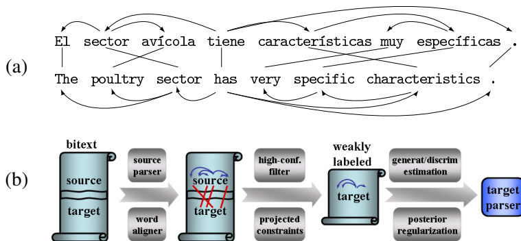
Figure 7: (a) An example word-aligned sentence pair with perfectly projected dependencies. (All dependency edges are conserved in this case.) (b) Overview of our grammar induction approach via bitext: the source (English) is parsed and word-aligned with target; after filtering, projected dependencies define constraints over target parse tree space, providing weak supervision for learning a target grammar.
