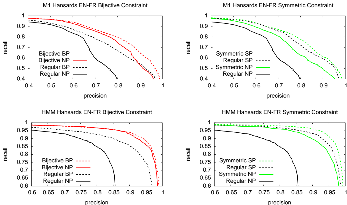
Figure 5: Precision vs Recall curves of both models using standard EM training (Regular) versus PR with bijective constraints (Bijective) and symmetry constraints (Symmetric) and different decoding types: decoding without any projection (NP), doing bijective projection before decoding (BP), and doing symmetric projection before decoding (SP). Data is 100k sentences of the Hansards corpus. Highest label in the legend corresponds to highest line in the graph, second highest label to second highest line, and so on.
