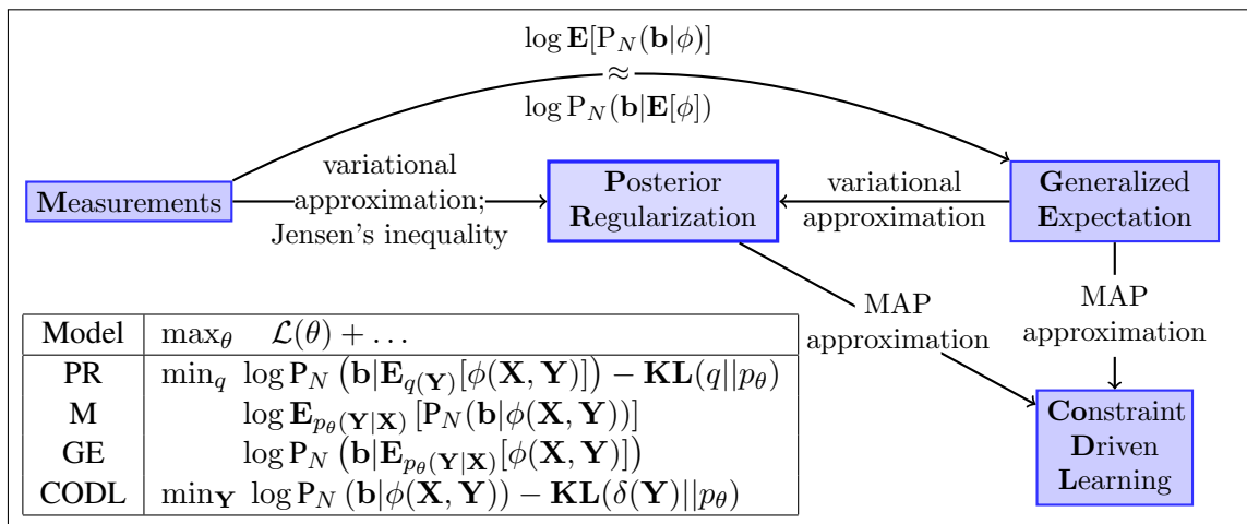
Figure 3: A summary of the different models. We use p_{\theta}(\mathbf{Y}|\mathbf{X}) to denote the model probability, q(\mathbf{Y}) to denote a proposal distribution, and \mathbf{P}_N for the noise model. The symbol \delta(\mathbf{Y}) denotes a distribution concentrated on \mathbf{Y} . The approximations are described in the text: \text{M} \rightarrow \text{GE} near Equation 35, \text{GE} \rightarrow \text{PR} near Equation 30, \text{PR} \rightarrow \text{CODL} at the end of Section 4.3.
