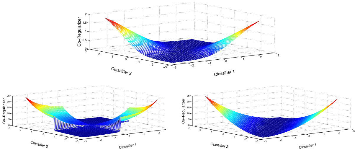
Figure 6: Different Loss Functions. Top : Bhattacharyya distance regularization. Bottom left : Exponential loss regularization. Bottom right : Least squares regularization.
