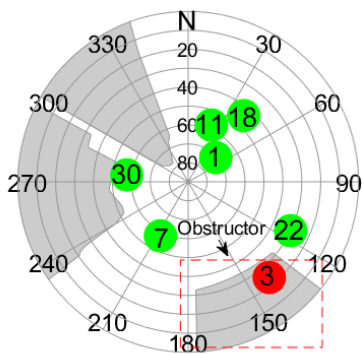
Fig. 17. Ray tracing result of PRN 3.
