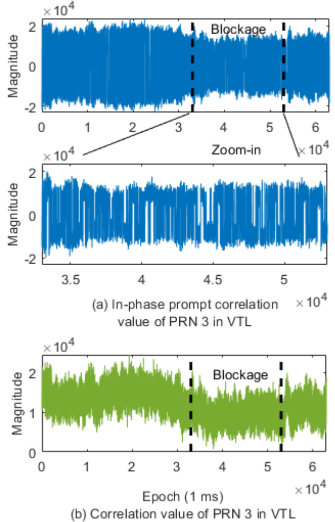
Fig. 20. Tracking results of PRN 3 in VTL. (a) In-phase prompt correlation value; (b) Correlation value of PRN 3.
