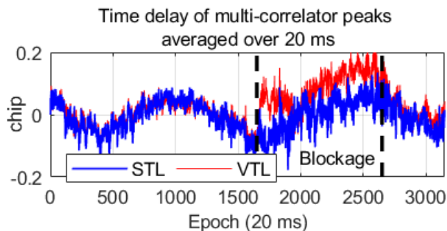
Fig. 23. Code discriminator output of PRN 3.
