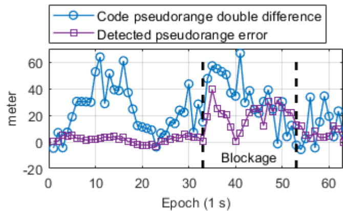
Fig. 24. Detected pseudorange error of PRN 3 with comparison to code pseudorange double difference.
