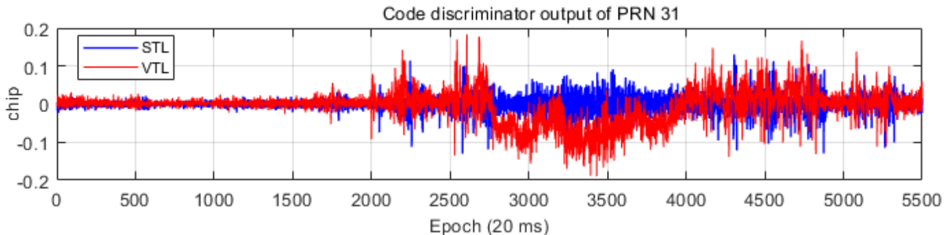
Fig. 10. Code discriminator outputs for PRN 31.
