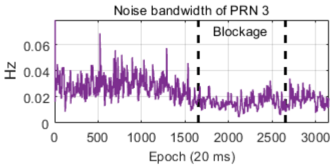
Fig. 21. Noise bandwidth of PRN 3 in VTL.
