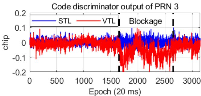
Fig. 22. Code discriminator output of PRN 3.
