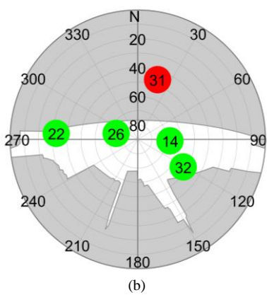
Fig. 8. Skyplots with building boundary information at (a) Points 1 and (b) 2.
