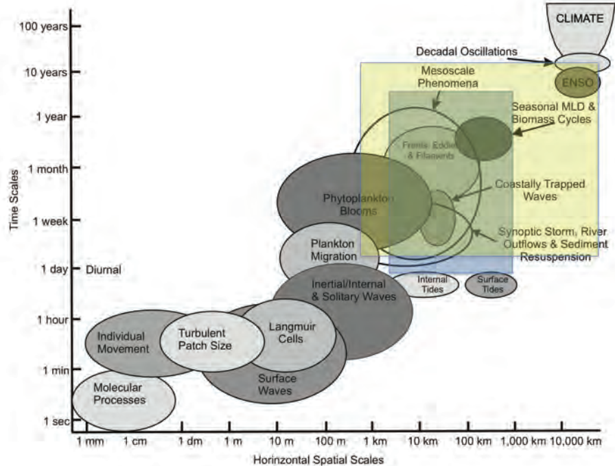
Figure 1.1 The spatio-temporal domain relevant to major physical and biological processes in the context of observations by remote sensing (shaded yellow) and profiling floats (shaded blue). The intersection between both spatio-temporal domains identifies the scales of oceanic processes that can be scrutinized using both remote (space and in situ ) approaches. For the open ocean, it encompasses processes that are essential for our understanding of the impact of physical forcing on the biogeochemical cycle of carbon. Adapted from Dickey (2003).
