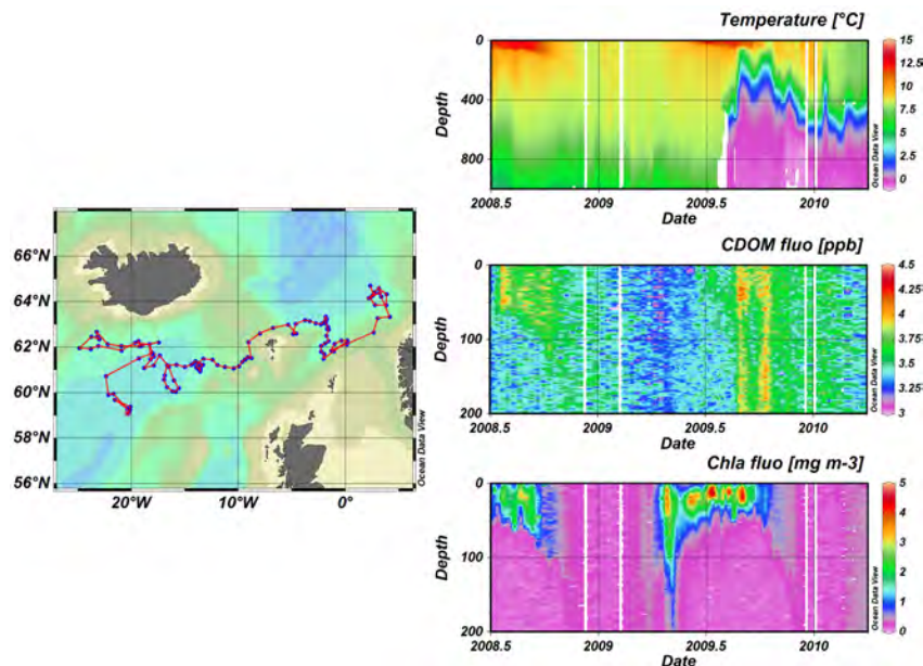
Figure 3.5 Time-series (22 months) of a PROVOR float equipped with a bio-optical package (ECO from Wetlabs) during its travel in Icelandic and Norwegian basins. The change of water masses is highlighted by the cold deep water, typical of Norwegian basin deep waters. This change is clearly traced by an enhancement of CDOM fluorescence. A sub-surface relative maximum in CDOM is also recorded at the beginning of the observational period, associated with high [Chla] ( \sim 2\text{-}4 \text{ mg m}^{-3} ) in the mixed layer (Claustre et al. unpublished data).
