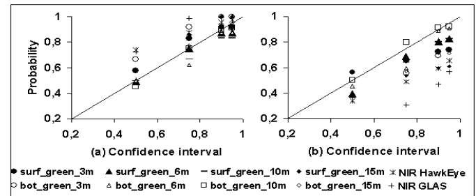
Fig. 3. a) Probability for an observed SNR to belong to a simulated SNR interval, b) Probability for a simulated SNR to belong to an observed SNR interval.
