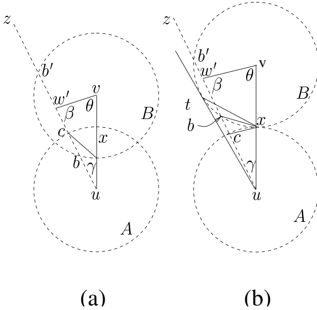
Fig. 12. Nodes are present at u , v , x , and w which is any point on \overline{uz} , with |\overline{uw}| > |\overline{uv}| . (a) Cases 1 and 2: node w is located either inside circle A or B . (b) Case 3: node w is between c and b but outside both A and B .
