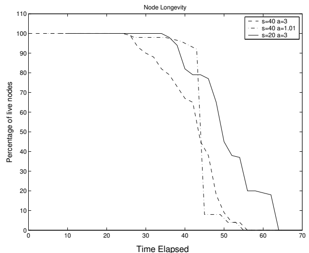
Fig. 11. Lifespan of network executing the clustering algorithm. There is a distinct knee in the curve for large dense clusters ( s = 40, a = 1.01 ), whereas sparse clusters ( s = 20, 40, a = 3 ) result in a graceful degradation of the network.
