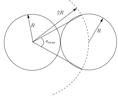
Fig. 4. Geometric interpretation of the maximal cone angle a = 2 \sin^{-1} \frac{\sqrt{15}}{8} : the angle subtended at the center of a circle from the intercepts of an adjacent circle with the same radius and a concentric circle with double the radius.
