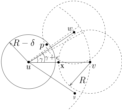
Fig. 5. Clusterhead uses a gap_{a+2\epsilon} criterion which makes its radius R - \delta , disconnecting cluster C_v .
