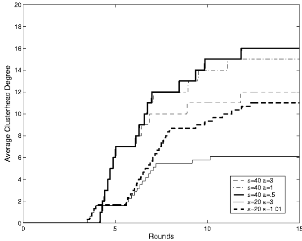
Fig. 8. Average degree of the clusterheads.
