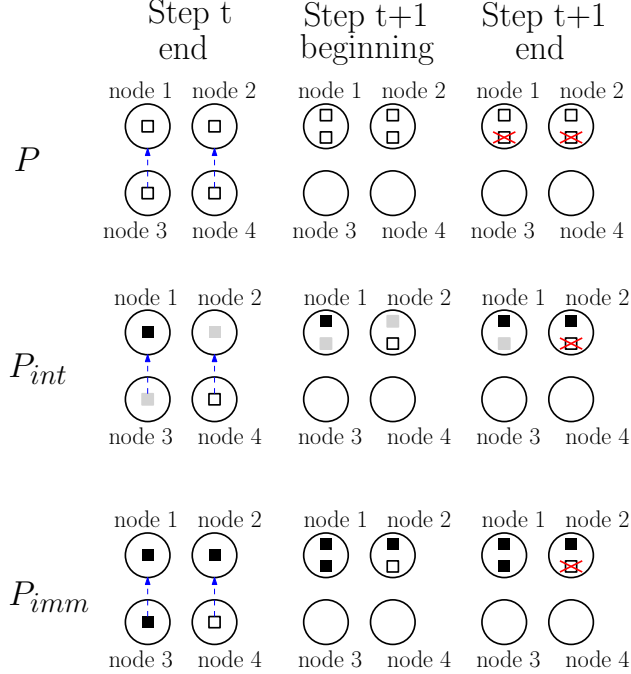
Figure 3: An illustration of couplings between the processes. The squares depict the random walks. Walks of \mathcal{G}_1 are coloured black and grey (phantom) and the nodes of \mathcal{G}_2 are white. The blue arrows denote the moving decisions. Observe that in P_{\text{int}} a phantom becomes alive (and a walk of \mathcal{G}_2 is labeled dead).
