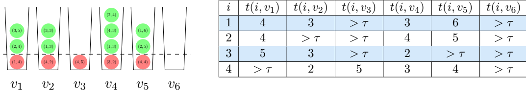
Figure 5: Illustration of the balls-into-bins configuration of k = 4 walks labeled 1, 2, 3, 4 into 6 vertices v_1, v_2, \dots, v_6 . In the illustration, a ball (i, t(i, u)) on bin u is good if there is at least one other ball with t(i, u) < t(j, u) (or t(i, u) = t(j, u) and i < j ). For each of the random walks 1, 2 and 3, there are at least two good balls, while for random walk 4 only one ball is good.
