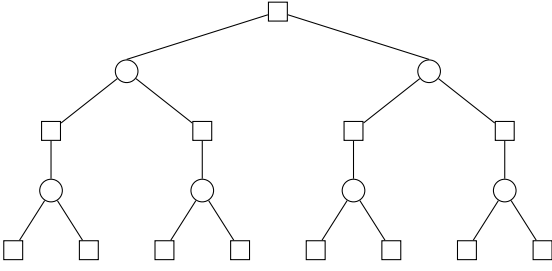
Fig. 4.1 A ((2), (3), 2) -tree rooted at the bin on top. Note that the 2-hop neighborhoods of the balls adjacent to the root are isomorphic. The leaf bins may have edges to balls outside the tree, which are not depicted.
