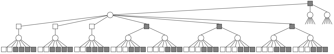
Fig. 4.2 A subtree of a ((2, 3), (3, 4), 2) -tree rooted at the bin on top. White bins have been contacted in the first round only, grey bins in the second. Note that (i) the 2-hop neighborhoods of the balls adjacent to the root are isomorphic, (ii) the neighborhoods of grey non-leaf bins are isomorphic, and (iii) the neighborhoods of white non-leaf bins are isomorphic. The further a node from the closest leaf, the larger the hop-distance for which the respective neighborhoods look identical. Again, leaf nodes may have been contacted by balls outside the tree, which is not depicted.
