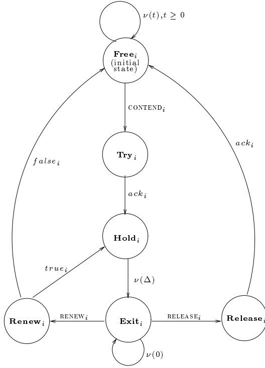
Figure 4: Well-formed interaction of process i and the \Delta -Lease object with renewals
