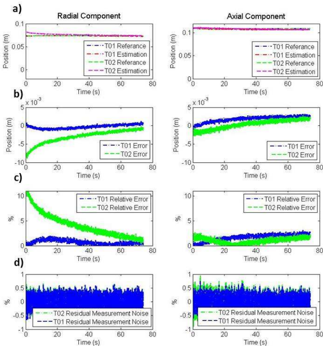
Fig. 9. Results for the steady state positional drift experiment (T01) and for the initialization error evaluation (T02) with an initialization error of 10mm. Both T01 and T02 results are evaluated for the radial (left column) and the axial (right column) component. (a) Reference position vs. estimation. (b) Absolute positional errors. (c) Relative positional errors. (d) Residual measurement noise. The azimuth error is presented in Fig. 12.
