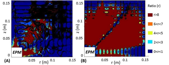
Fig. 5. The ratio of relative errors of the single dipole model to the interpolation model for the radial (A) and axial (B) magnetic field components. Black regions stem from visualization artifacts due to oscillations in the ratio from 3 to 8 times.
