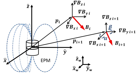
Fig. 1. Schematic representation of the source of magnetic field (External Permanent Magnet (EPM) in figure) and two sequential positions (i.e., \mathbf{p}_i and \mathbf{p}_{i+1} ) of the capsule to be localized. The capsule orientational angles yaw and pitch are referred to as \alpha and \beta , respectively.
