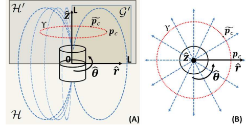
Fig. 3. Schematic view of the magnetic field distribution for a cylindrical axially-magnetized permanent magnet. (A) View of the \mathcal{H} planes, its subset \mathcal{H}' and the domain \mathcal{G}' , (B) shows the radial distribution of the magnetic field on the plane [\hat{r}, \hat{\theta}] .
