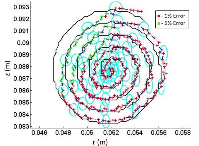
Fig. 6. Simulated motion of a capsule along a spiral trajectory in the center of \mathcal{G}' . The black line represents the reference trajectory, while the crossed line shows the capsule position estimated by applying the Jacobian-based iterative method. The cyan ellipses represent the ellipsoid of localization uncertainty due to magnetic field sensor noise. Colors in the crossed line express the relative error in position detection for the radial component.
