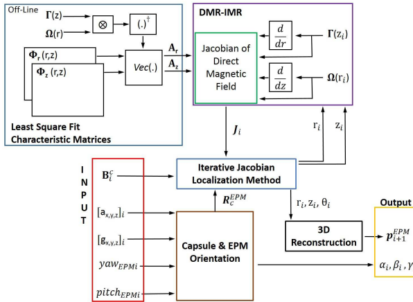
Fig. 2. Block diagram of the proposed iterative algorithm for WCE pose detection. In the diagram are displayed system input, output, Jacobian of the MDR, 3D reconstruction, and the off-line least square fit calibration, which leads to the characteristic matrices \mathbf{A}_r and \mathbf{A}_z .
