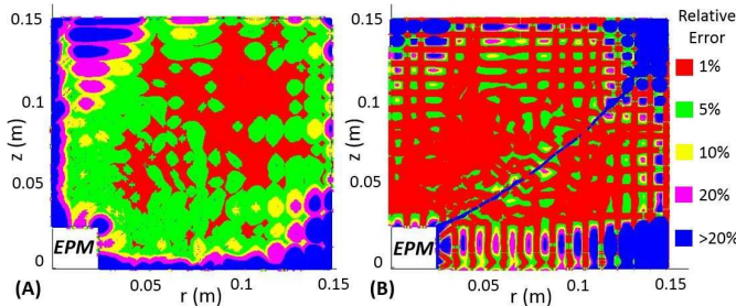
Fig. 4. Relative error for the radial (A) and axial (B) magnetic field estimated by the MDR within \mathcal{G}' .
