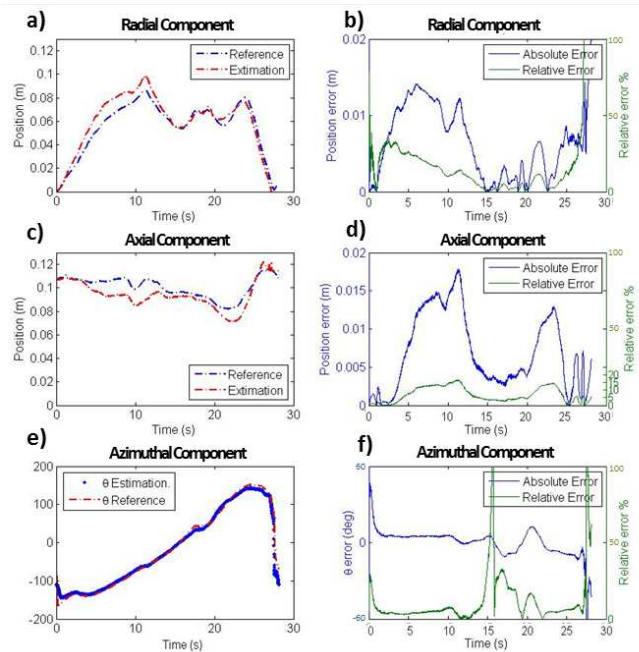
Fig. 12. Typical trends for the radial (a), the axial (c) and the azimuth (e) component during the final experiment, and related absolute and relative errors (b, d, and f, respectively).
