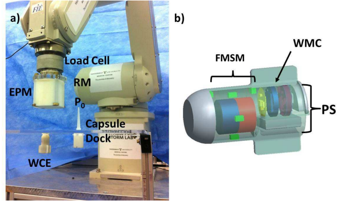
Fig. 7. Experimental platform: a) Robotic Manipulator (RM) and External Permanent Magnet (EPM). b) Visual rendering of the Wireless Capsule Endoscope (WCE) and its internal components, where FMSM is the Force and Motion Sensing Module, WMC is the Wireless MicroController and PS is the Power Supply.
