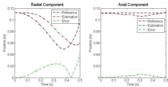
Fig. 10. Position estimation results during the positional lag trial with uniform acceleration of 1.984 \frac{m}{s^2} .
