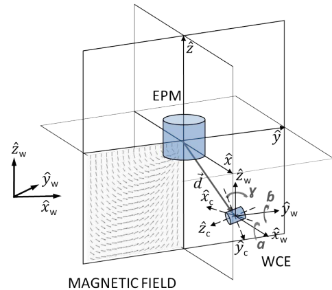
Fig. 8. Schematic representation of the global frame, EPM frame and capsule frame. The capsule orientation angles [\alpha, \beta, \gamma] are shown with respect to the global frame.
