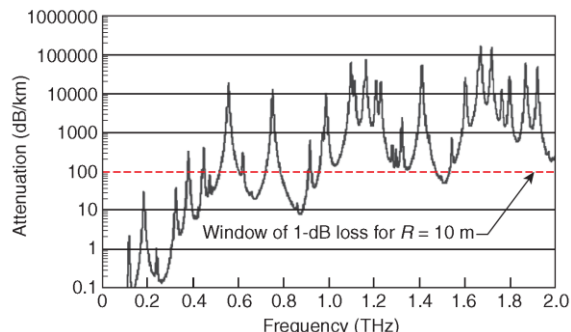
Fig. 7. Atmospheric attenuation in the THz frequency range [148].
