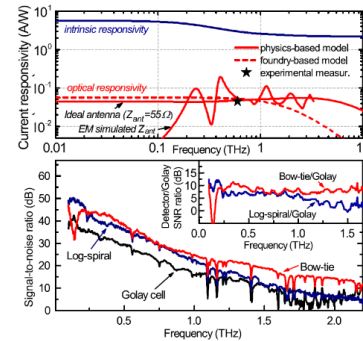
Fig. 4. Top: simulated and measured current responsivity vs. radiation frequency for TeraFET at Vg=0.45V. Black star denotes the responsivity of the TeraFET with a bow-tie antenna measured at 600 GHz. Bottom: comparison of the frequency-dependent SNR of the THz detectors (Vg=0.45V) and the comparison with the Goley cell inserted (reproduced from [110]).
