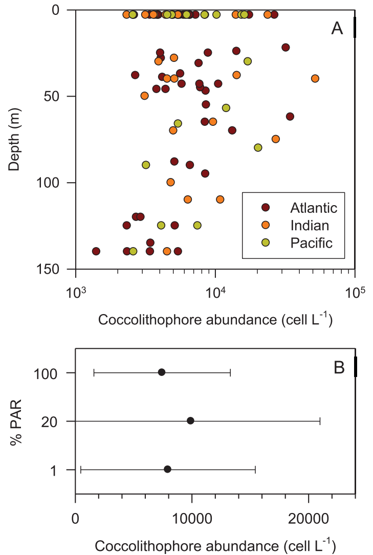
Fig. 5. Cocolithophore abundance ( \text{cell L}^{-1} ) over depth for each ocean and mean values for each PAR level with all data combined. Bars represent the standard deviation.
