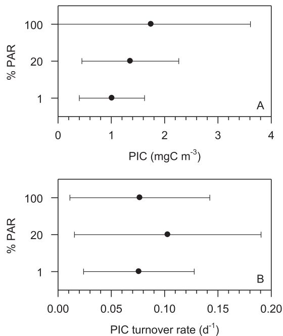
Fig. 6. Mean concentration ( \text{mgC m}^{-3} ) and turnover rate ( \text{d}^{-1} ) of particulate inorganic carbon (PIC) at each PAR level with data from the Atlantic and Indian oceans.
