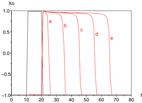
Fig. 8. The Neural One-Shot's output pulse width can easily be adjusted by varying timing parameter w_f . Shown are output transients for the following values: a) -0.9959 , b) -0.6087 , c) -0.5777 , d) -0.5692 , and e) -0.5657 .
