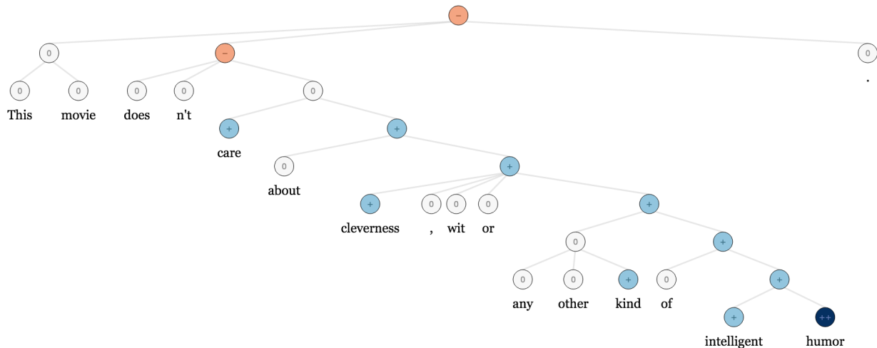
Figure 9: RNTN applied on the dependency tree of the sentence “This movie doesn’t care about cleverness, wit or any other kind of intelligent humor”.
