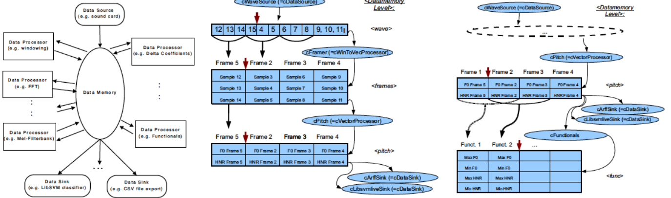
Figure 6: The OpenSMILE framework.
