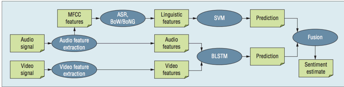
Figure 10: Hybrid fusion for multimodal sentiment analysis in YouTube videos as proposed by [? ].
