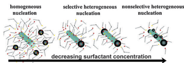
Fig. 14 Mechanism for surfactant-controlled Co NC heteronucleation and growth on TiO 2 nanorod seeds. Adapted with permission from ref. 63. Copyright 2007 American Chemical Society.
