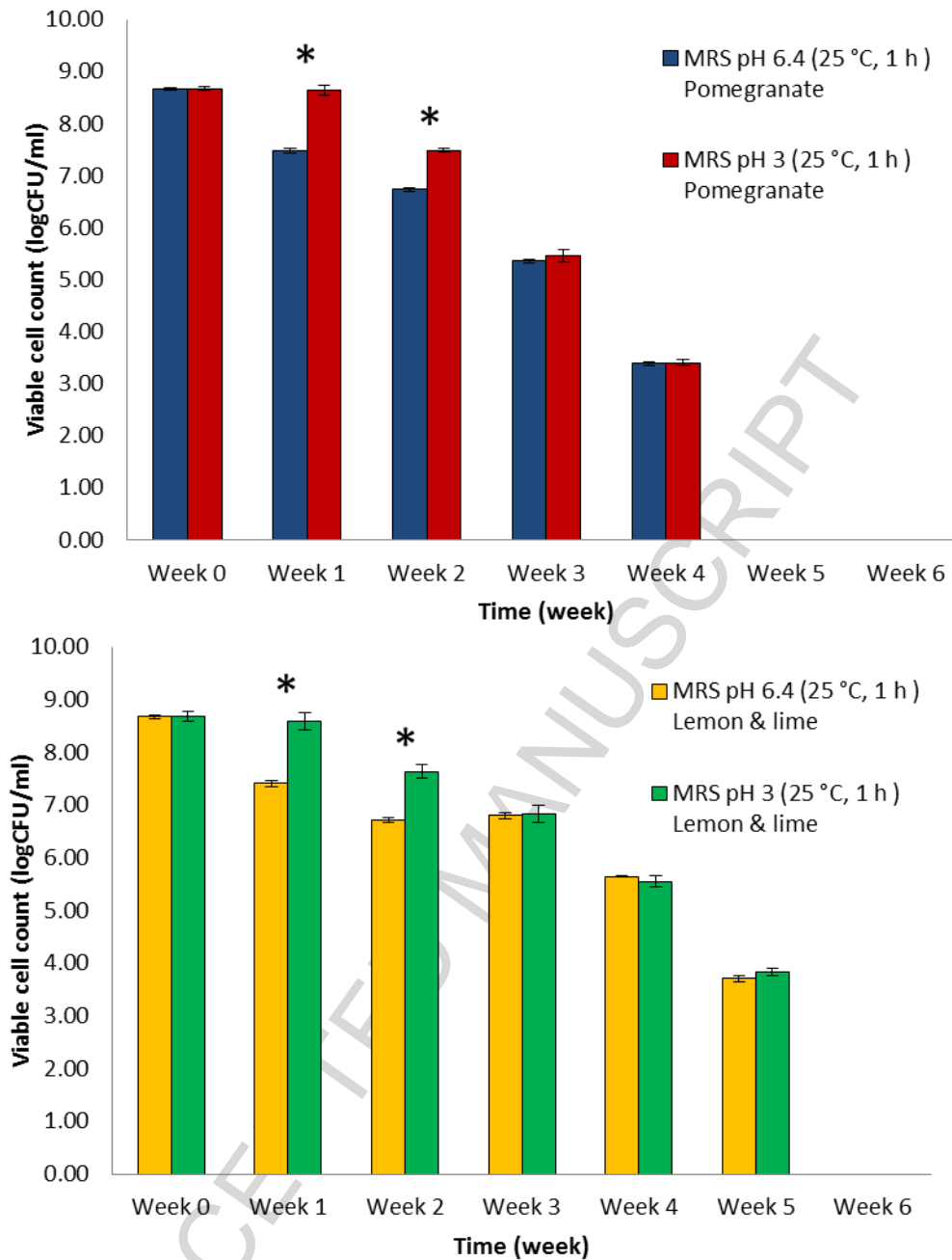
Figure 2. Survival of L. plantarum NCIMB 8826 during refrigerated storage in pomegranate (A), and lemon & lime (B) after pre-treatment in acidified MRS (pH 3, 25 °C, 1 h) and in unmodified MRS (pH 6.4, 25 °C, 1 h). Results are expressed in mean \pm SD (n=3). Significant differences in cell viability between acidified cells (pH 3) and control cells (pH 6.4) at specific time point were determined by paired t-test. Asterisk indicates significant differences.
