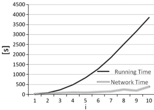
Fig. 7 Network Time and Running Time for the family S^{10} of networks
