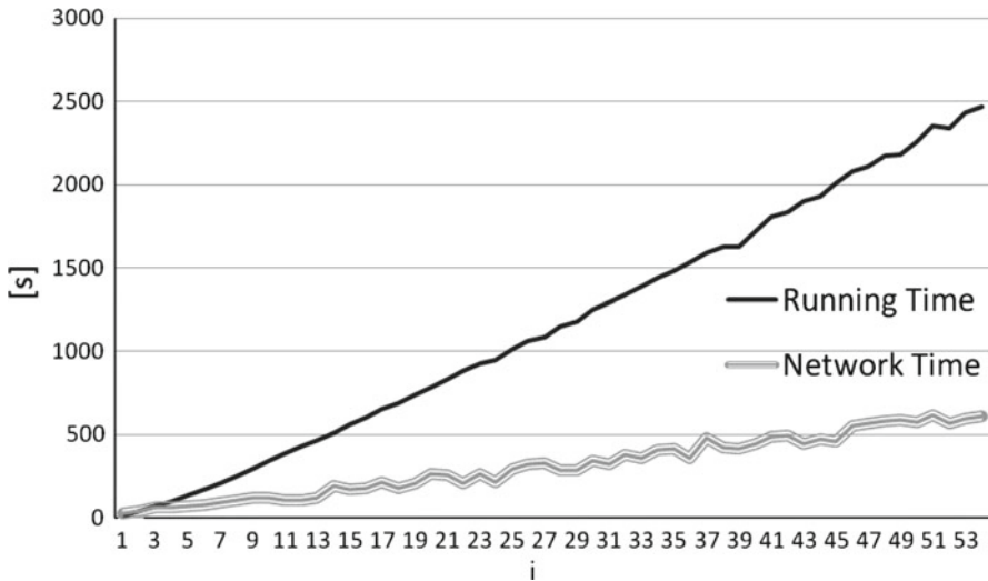
Fig. 5 Network Time and Running Time for the family L^{53} of networks
