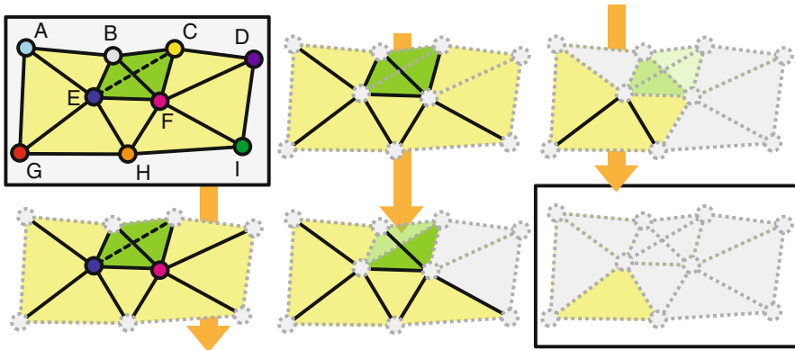
Fig. 4 From top left , to bottom right , following the arrows : a collection of sensors and the associated S-complex, the S-complex after removing the fence, the fence complex after removing the consecutive free collections of S-reduction pairs, the final reduced S-complex
