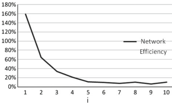
Fig. 8 Efficiency of the network for the family S^{10} of networks
