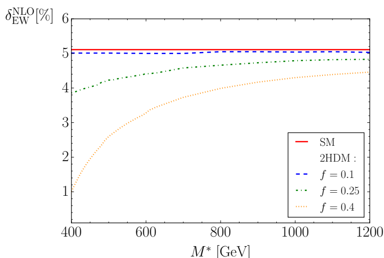
Figure 2. EW NLO corrections to Higgs-boson production in gluon fusion as a function of the scale M^* . The values of M_{H_h} , M_{H_a} , M_{H^\pm} and M_{S_b} are chosen according to eq. (6.8). The solid line represents the SM. The dashed, dashed-dotted, and dotted lines correspond to f = 0.1 , f = 0.25 and f = 0.4 .
