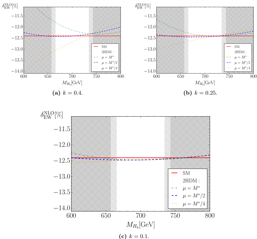
Figure 3. NLO percentage EW corrections to the integrated cross section of pp \rightarrow Hl^+l^- + X as a function of the heavy Higgs-boson mass M_{H_h} for three different scenarios, which differ by the value of c_{\alpha\beta} parametrized according to eq. (6.10). The solid line indicates the SM result. The dashed-dotted, dashed, and dotted lines show the percentage correction in the 2HDM (normalized to the 2HDM Born) for different values of the renormalization scale \mu = M^*, M^*/2, M^*/4 . The heavy masses M_{H_a} = M_{H^\pm} = M_{s_b} = M^* = 700 GeV and t_\beta = 2 are kept constant. The bright grey band represents the region 0.4 \leq f \leq 0.5 [see eq. (6.7)] and the dark grey band the region f > 0.5 .
