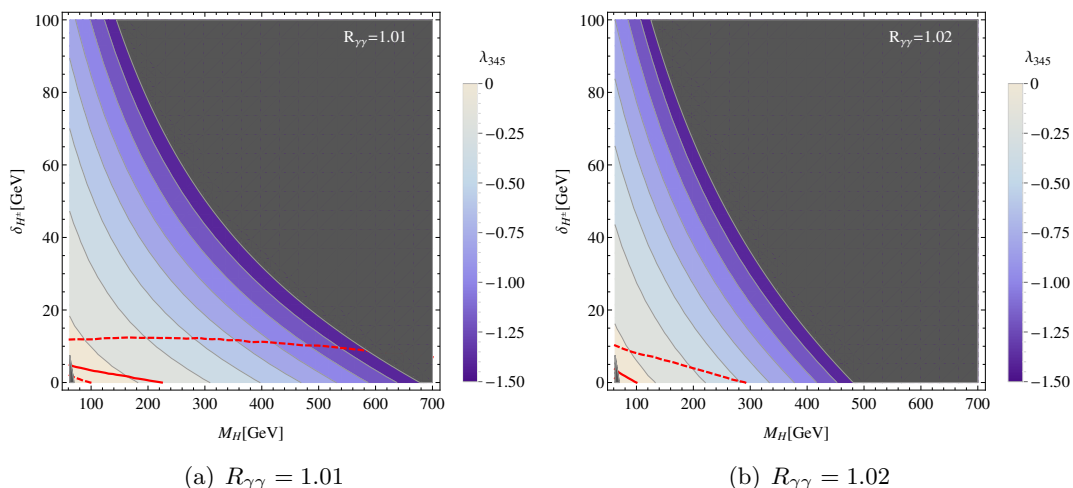
Figure 7. Allowed regions in (M_H, \delta_{H^\pm}) plane for two values of R_{\gamma\gamma} : 1.01 (left panel), 1.02 (right panel). Dark grey region is excluded due to LEP bounds (left lower corner) and the vacuum stability/unitarity constraints (2.8) (right upper corner). Red lines show bounds from XENON100 (solid for f_N = 0.326 , dashed for f_N = 0.14 and f_N = 0.66 ) — region above this line is excluded, if we assume that the dark scalar H constitutes all dark matter relic density.
